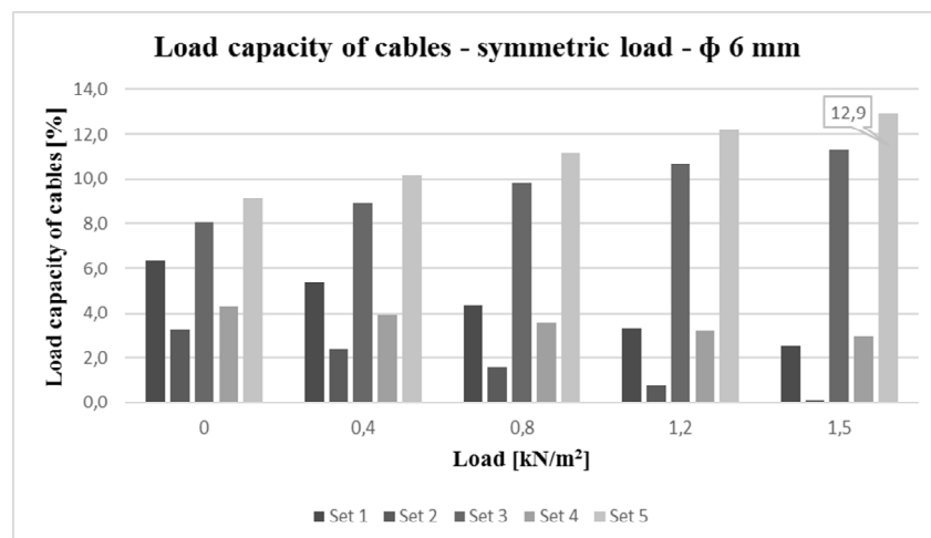
Fig. 7. Load capacity of cables – ϕ 6 mm
