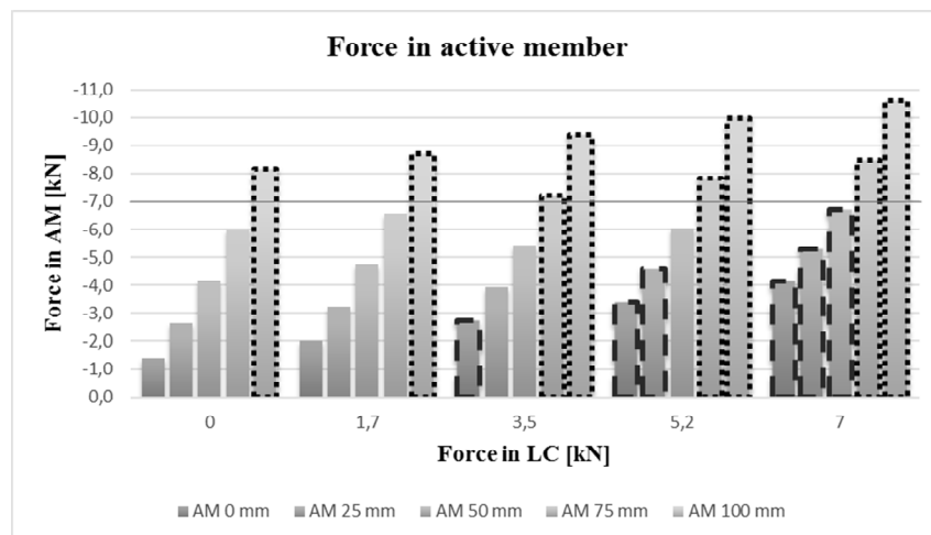
Fig. 9. Force in active member – \phi 4 mm
