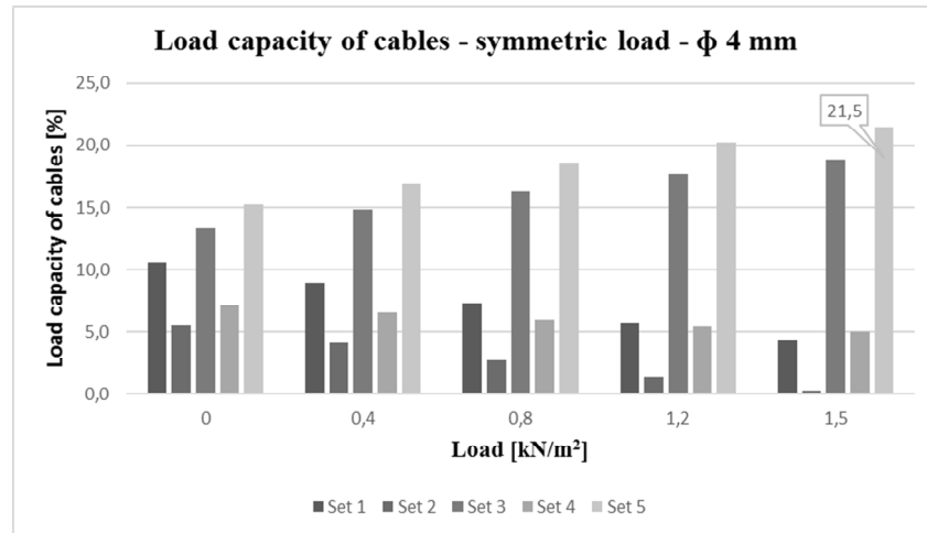
Fig. 6. Load capacity of cables – ϕ 4 mm
