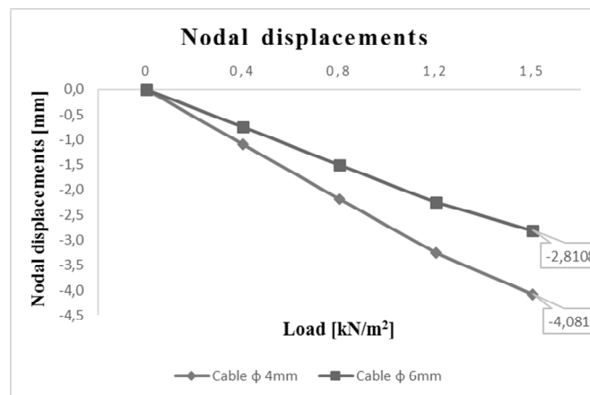
Fig. 5. Nodal displacements
