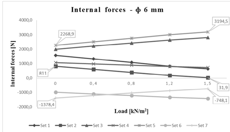
Fig. 4. Internal forces – \phi 6 mm
