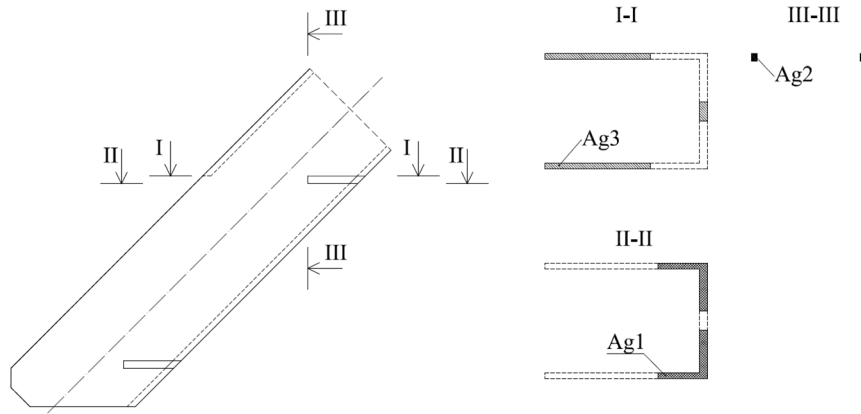
Fig. 5. Tension brace view – top connection
