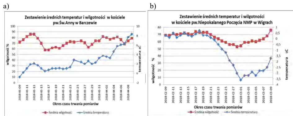
Fig. 6. Temperature and dampness levels as a function of time) a) temperatures and humidity of interior air - Barczewo (2) b) temperatures and humidity of interior air – Wigry
