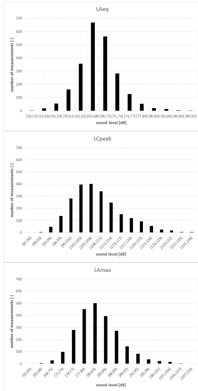
Fig. 3. A-weighted equivalent sound level, C-weighted peak sound level and A-weighted maximum sound level L_{Amax} registered on scaffoldings in Warszawa
