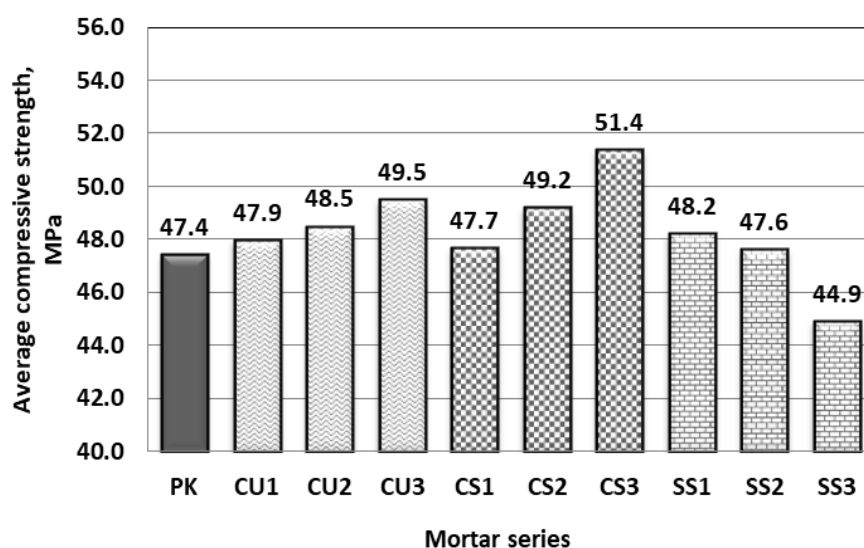
Fig. 2. Average compressive strength of investigated cement mortars
